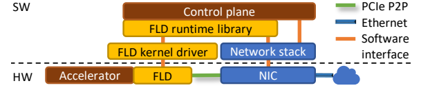
Figure 5: FLD high-level software design.
