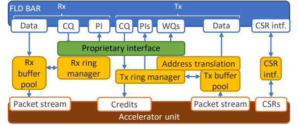
Figure 3: FLD hardware functional diagram.
