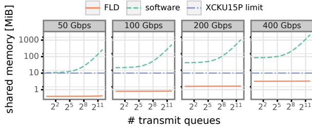
Figure 4: Driver memory requirements w/o FLD optimizations. XCKU15P—on-chip memory on our prototype’s FPGA.
