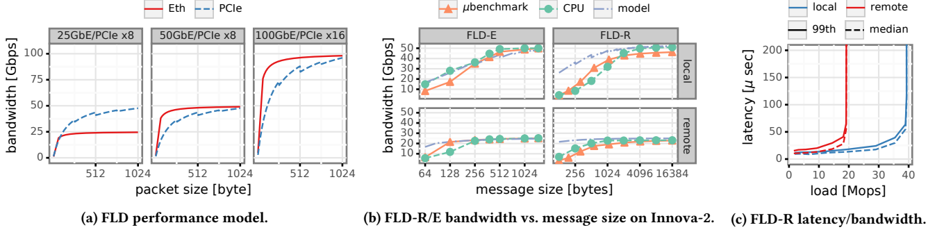
Figure 7: FLD microbenchmarks.
