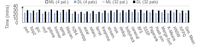
Figure 13: Profiling time for K-Means vs DL-assisted K-Means
