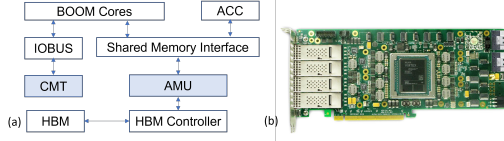
Figure 10: (a) Diagram of the prototyping system; (b) Photo of the FPGA prototyping platform with integrated HBM devices
