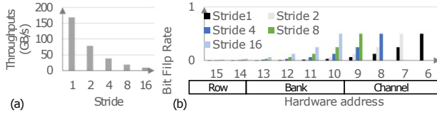
Figure 3: (a) HBM throughput with different stride using the default address mapping; (b) Bit flip distribution for different stride using the default address mapping
