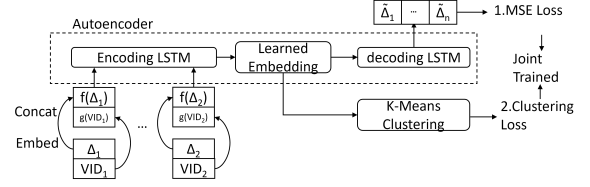
Figure 9: The embedding LSTM model.
