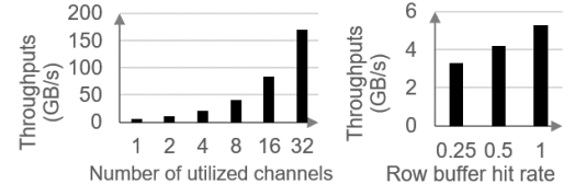
Figure 1: Comparing HBM throughput for different number of channels and row buffer hit rate
