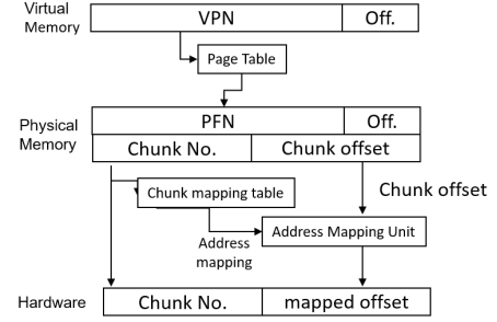
Figure 5: Chunk-based address mapping management
