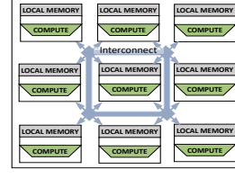
Figure 2: Homogeneous CGRA
