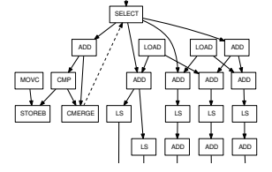
Figure 3: Snippet of DFG
