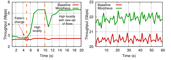
Figure 9: (a) Single core throughput over time with Morpheus on the Router use case, with dynamically changing traffic patterns, and (b) with a CAIDA [22] trace.
