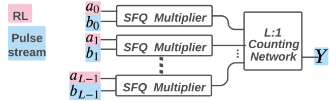
Figure 15: Proposed U-SFQ Dot Product Unit.
