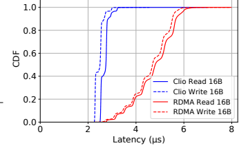
Figure 7: Latency CDF.
