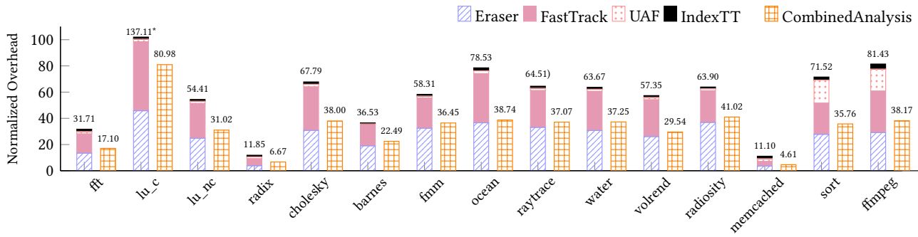
Figure 5: Combined Analysis of Eraser, FastTrack, Use After Free and Taint Tracking(*: bar compressed).
