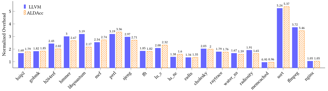
Figure 3: LLVM MSan VS ALDACC MSan.
