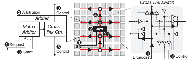
Figure 19: CryoBus overview and working mechanism
