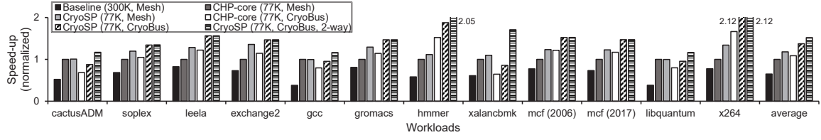
Figure 24: Single-thread performance of SPEC 2006 and 2017 workloads with an aggressive stride prefetcher
