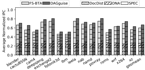
Figure 10: Average Normalized IPC of two DocDist, two DNA, and four SPEC processes on an eight-core system.
