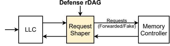
Figure 3: DAGguise overview.
