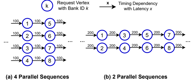
Figure 6: Example rDAGs used in DAGguise, derived from rDAG templates.
