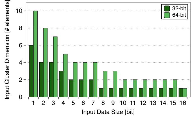
Figure 2: Maximum input-cluster dimension achievable on 32-bit and 64-bit architectures, for data sizes ranging from 1-bit to 16-bit. The input-cluster dimension is defined as the number of elements that can be packed in a single register, following the binary segmentation constraints.
