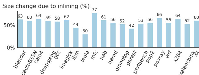
Figure 1: This figure shows that inlining is a critical compiler optimization. It depicts size improvement due to inlining for the SPEC2017 benchmark suite (not including the Fortran-only benchmarks) for LLVM's -Os optimization level; in the best case, enabling inlining results in up to 3× size improvement. For example, for the benchmark "leela", the resulting binary size with inlining enabled is 30% of that with inlining disabled when compiling at LLVM's -Os.
