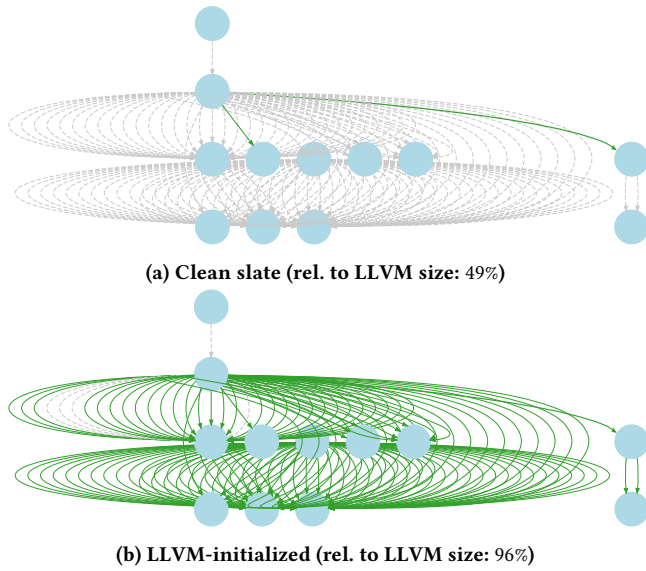
Figure 13: imgick:decorate.c : example call graph which fares better with clean slate autotuning.
