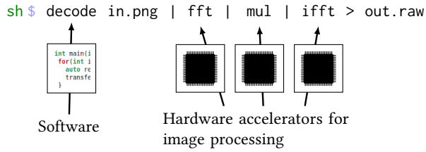
Figure 2: Combination of software (decode) and hardware accelerators (fft, mul, and ifft) in M 3 x's shell.
