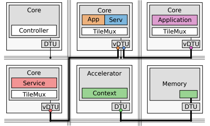
Figure 3: System architecture of M 3 v. The DTU endpoints at the end of communication channels correspond to the activity that owns the endpoint.
