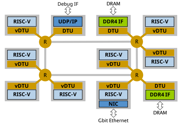
Figure 4: The M 3 v hardware platform with eight RISC-V tiles, two memory tiles, and one debug tile. The tiles are connected via a NoC with four routers (R).
