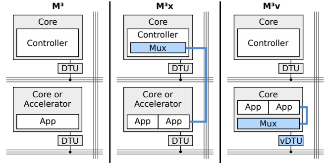
Figure 1: Tile multiplexing on M 3 (no multiplexing), M 3 x (all tiles can be multiplexed using a single centralized OS tile), and M 3 v (general-purpose tiles can multiplex themselves). Each of the lower tiles can exist multiple times in a real platform.
