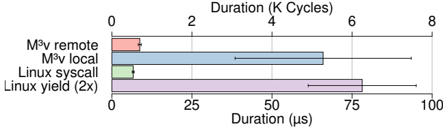
Figure 6: Local/remote communication on M 3 v and similar primitives on Linux as a reference.
