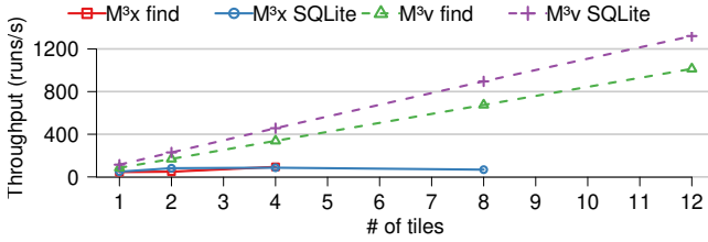
Figure 9: Scalability of context-switch-heavy applications on M³x and M³v with tile multiplexing.
