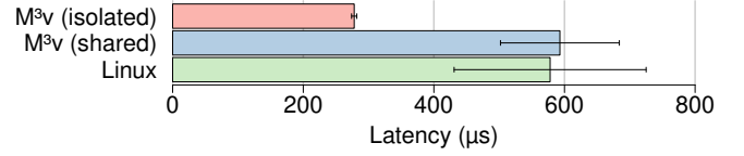
Figure 8: UDP latency comparison. The results without tile sharing (“isolated”) cannot be compared to Linux, because in contrast to Linux, M 3 v uses multiple tiles.
