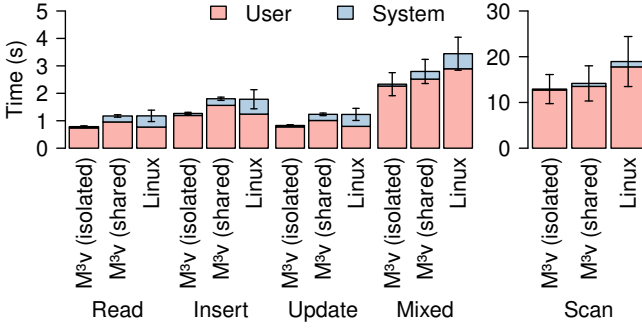
Figure 10: Cloud service in comparison to Linux. The results without tile sharing (“isolated”) cannot be compared to Linux, because in contrast to Linux, M 3 v uses multiple tiles.
