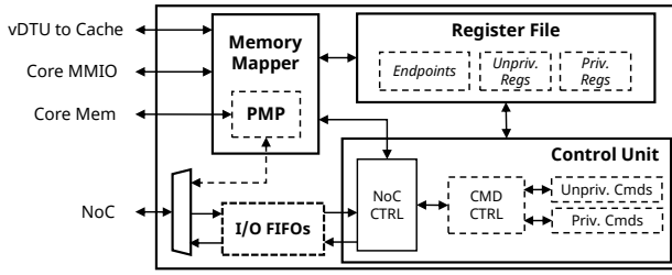
Figure 5: Hardware implementation of the vDTU. Dashed blocks and arrows indicate optional components.
