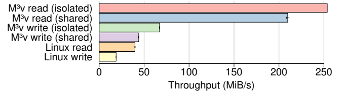
Figure 7: File read/write throughput comparison. The results without tile sharing (“isolated”) cannot be compared to Linux, because in contrast to Linux, M 3 v uses multiple tiles.
