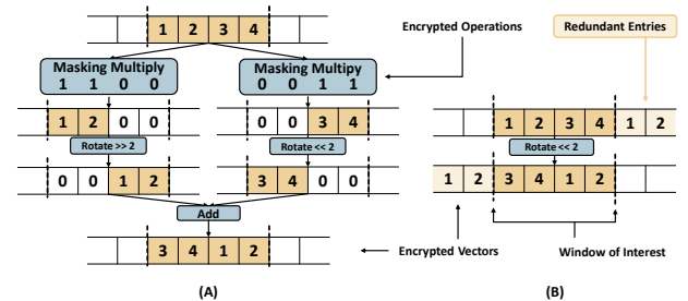
Figure 4: Encrypted windowed rotation using arbitrary permutation (A) and rotational redundancy (B). Rotational redundancy is a novel way of packing input values before encryption that allows for fewer encrypted operations.
