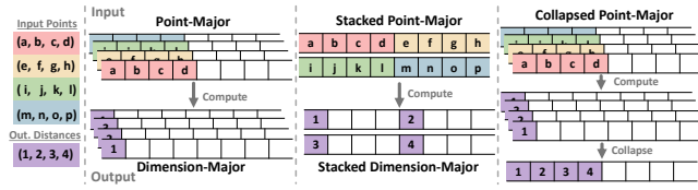
Figure 9: Encrypted vector packing for distance calculations.
