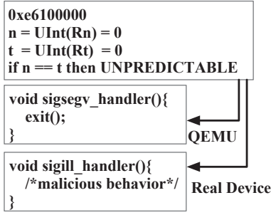
Figure 7: Inconsistent instruction can prevent the malicious behavior being detected by emulators
