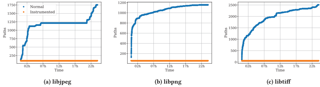
Figure 9: The result of Anti-Fuzzing experiment on three libraries. The blue lines show the coverage over 24 hours of fuzzing. The orange line shows the coverage for instrumented binaries, which cannot increase due to failed executions of QEMU.
