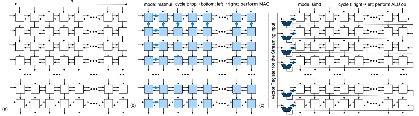
Figure 5: This figure shows the traditional systolic array design with dimensions n \times n in (a), the systolic array performing a matrix multiplication in matmul mode depicted in (b), and the systolic array performing a SIMD ALU operation in simd mode illustrated in (c). In order to perform SIMD ALU operations using the systolic array, a column of n ALUs need to be implemented. To eliminate unnecessary stall, pipelining interleaved matrix multiplication and matrix SIMD ALU operations informed our design to have the systolic array act as a large column left-rotator, producing n SIMD operation results per cycle.
