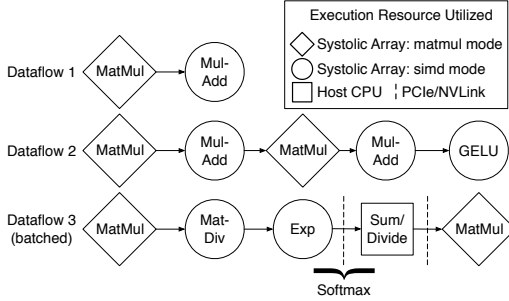
Figure 6: Across model layers, we found three major operation sequences are executed for around 90% of the total inference time. If each operation sequence can be executed in a dataflow-esque fashion on the accelerator without communicating with the host, it would maximize the efficiency of the design. Note that Dataflow 3 still has a softmax operation that requires host-accelerator communications, trading performance for hardware simplicity.
