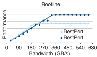
Figure 20: Empirical roofline for BestPerf and BestPerf+ designs. As the different heterogeneous components of ProSE become compute-bound, the BestPerf and BestPerf+ designs creep towards saturation.
