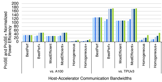
Figure 19: Power efficiency of ProSE over NVIDIA A100 GPU and TPUv3 when evaluated with different link bandwidths. ProSE is a lot more power-efficient than TPUv3 (two orders of magnitude more efficient) due to the elimination of the large and power-hungry Unified Buffer.
