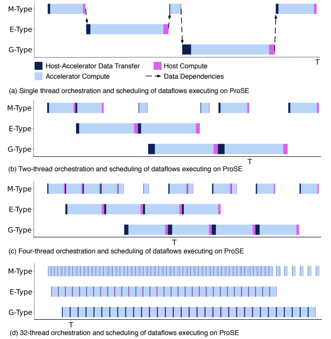
Figure 8: ProSE uses an orchestration and scheduling mechanism that maps software threads to systolic arrays. Multi-threading enables parallel execution of systolic arrays, significantly improve system throughput and efficiency.
