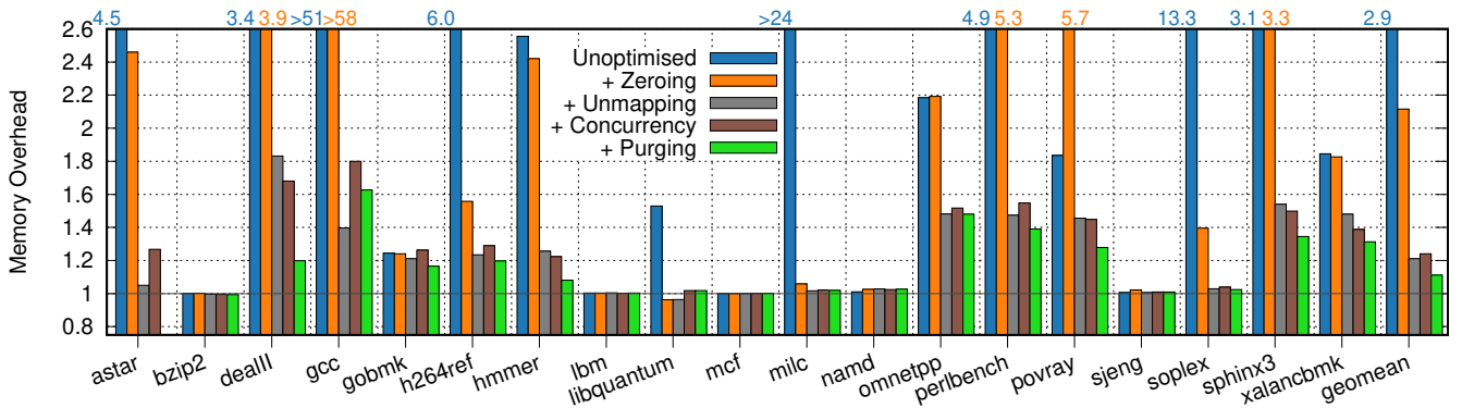
Figure 16: Average memory overhead under different optimisation levels (Section 4). Values with ‘&gt;’ failed from lack of DRAM.
