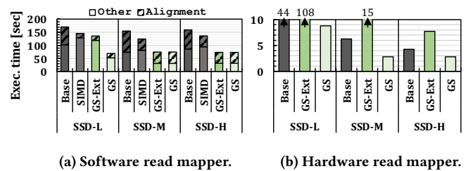
Figure 9: GenStore-EM performance under different SSDs.
