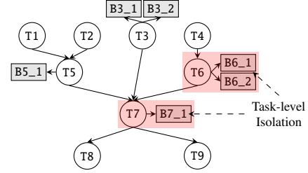
Fig. 4. Hierarchical addressing for the job in Fig. 3. Jiffy provides task-level resource isolation for far-memory under each task address-prefix (§3.1). Note that block addresses are only assigned to address-prefixes with currently allocated blocks; for tasks T1, T2 and T4, blocks are not stored in Jiffy, but read from persistent storage.
