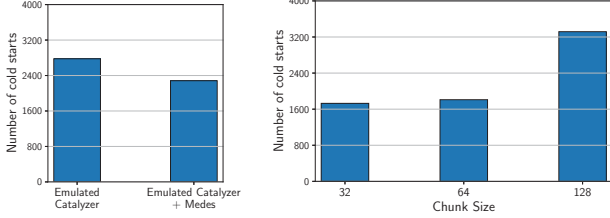
Figure 13. Integrating Medes with Catalyzer. Figure 14. Sensitivity to the Chunk Size Medes.
