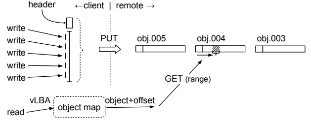
Figure 3. Log-structured block store. Writes are batched and written to immutable objects; reads are routed by an in-memory map. Garbage collection is not shown.
