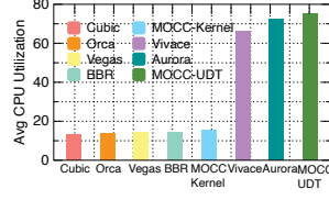
Figure 17. CPU Overhead of different CC schemes
