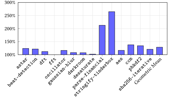
Figure 8. Chrome overhead using the Kraken benchmarks.
