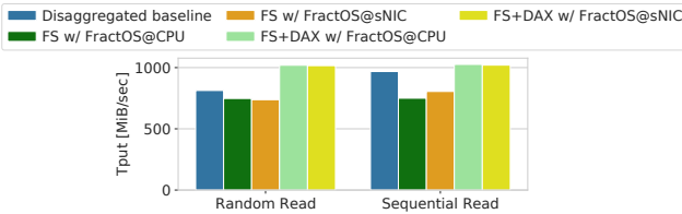
Figure 11. Throughput of random and sequential reads with 1024 KiB block size and 4 requests in flight (Higher is better).
