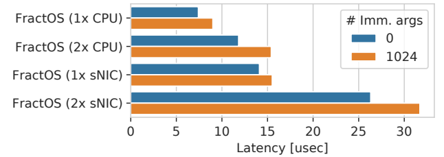
Figure 6. Latency of invoking a two-way Request (i.e., RPC) between Processes placed on one (1×) or two (2×) nodes (Shorter is better).
