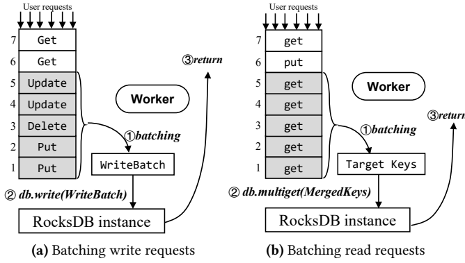
Figure 10. Opportunistic batching mechanism on RocksDB.
