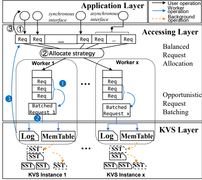
(a) p 2 KVS framework overview
