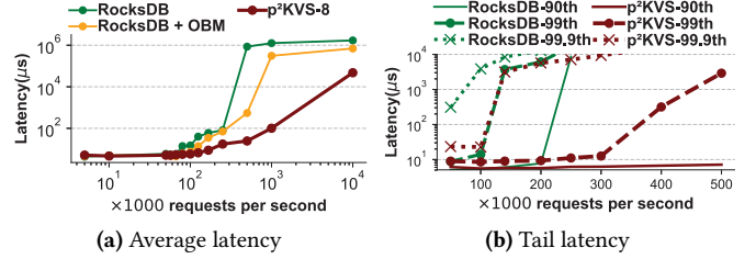
Figure 13. Write latencies as a function of different request intensities. "RocksDB + OBM" in (a) denotes a single RocksDB instance with the opportunistic batching mechanism.
