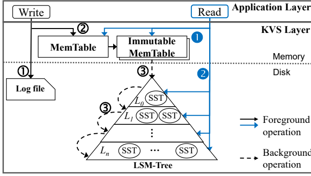
Figure 2. The main components of LSM-tree based KVS and the processing flow of KV write and read requests. ① Write-ahead logging. ② MemTable Index updating. ③ LSM-tree compaction. ① Search in MemTables. ② Search in LSM-tree.
