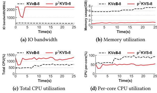
Figure 21. Hardware utilizations of p 2 KVS and Kvell under random write workloads.
