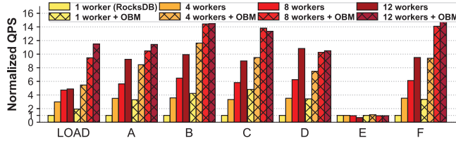
Figure 17. p^2 KVS sensitivity to the number of workers and OBM. The single-worker configuration is equivalent to RocksDB. All throughputs are normalized to RocksDB. Solid-colored and patterned bars are used to indicate OBM being disabled and enabled, respectively.
