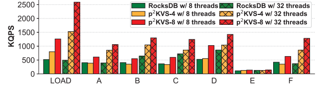
Figure 16. Throughputs under YCSB workloads.
