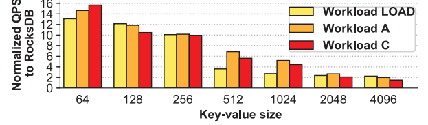
Figure 18. p^2 KVS sensitivity to key-value size.
