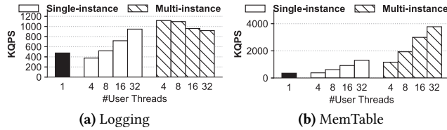
Figure 8. Throughput of different parallelizing schemes on the WAL and MemTable process respectively. MemTable inserting and indexing are disabled when testing WAL logging, and vice versa.
