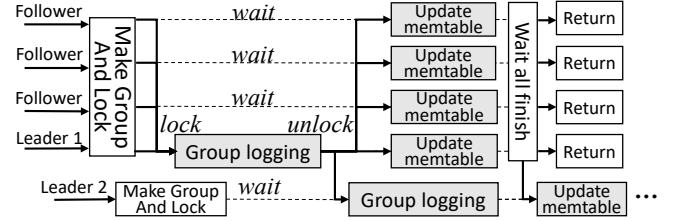
Figure 3. RocksDB concurrent write process.
