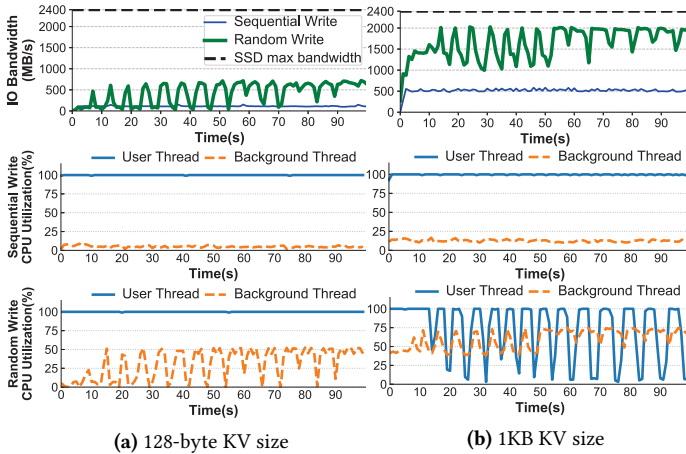
Figure 4. RocksDB IO bandwidth and CPU utilizations. A user thread continuously inserts 100M KV pairs sequentially and randomly, respectively, on an Optane SSD.
