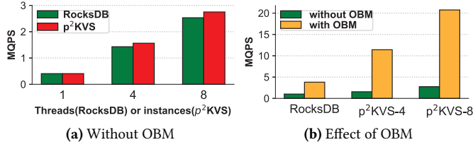
Figure 14. Throughput of point query.
