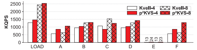
Figure 20. Overall performance of KVell and p^2 KVS.
