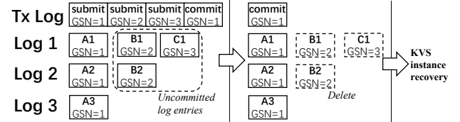
Figure 11. An example of transaction crash recovery.
