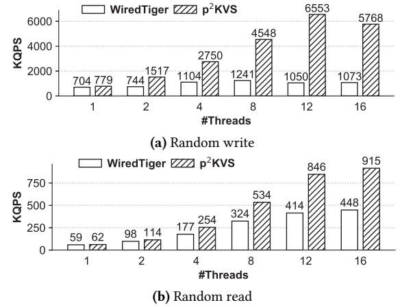
Figure 23. Performance of p 2 KVS on WiredTiger. The number of instances of p 2 KVS is equal to the number of threads.
