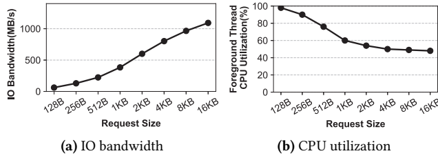
Figure 7. The effect of write request batching mechanism. The async-logging approach is enabled.
