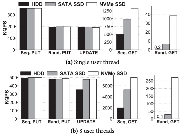
Figure 1. RocksDB single-threaded and multi-threaded throughput performance. HDD: WDC WD100EFAX 10TB, SATA SSD: Samsung 860 PRO 512 GB, NVMe SSD: Intel Optane 905p 480 GB. The hardware platform is equipped with two 22-core CPUs. The KV size is 128-byte.
