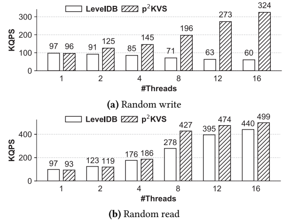
Figure 22. Performance of p 2 KVS on LevelDB. The number of instances of p 2 KVS is equal to the number of threads.
