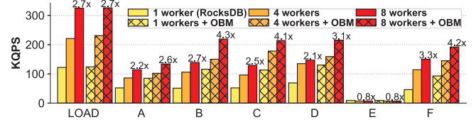
Figure 19. p^2 KVS performance at key-value size of 1KB.
