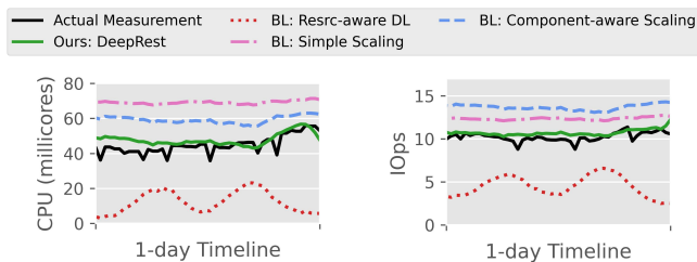
Figure 18. The estimation of two resources given the query API traffic in Figure 13c.
