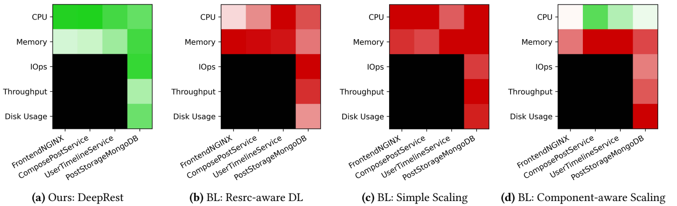
Figure 12. The estimation quality heatmaps on four components (columns) and five resource types (rows) in the social network. The green color represents accurate prediction while the red color indicates inaccurate estimation. IOps, throughput, and disk usage are inapplicable in stateless components and marked in black. DeepRest offers the most stable and accurate estimation compared with all other approaches.
