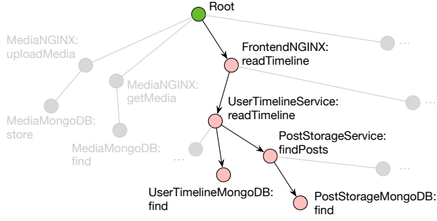
Figure 5. The execution topology graph highlighted with the invocation path of the example trace in Figure 3.
