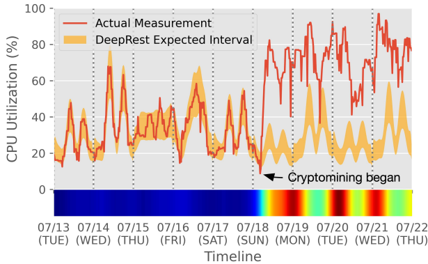
Figure 20. Using DeepRest to conduct application sanity checks to identify cryptojacking attacks.
