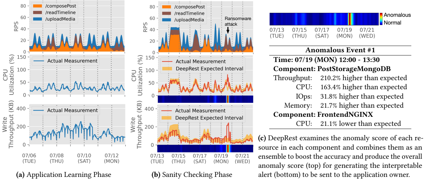
Figure 19. DeepRest (a) takes the API traffic and the corresponding resource utilization to learn the application and (b) estimates the expected utilization interval of each resource for sanity checks. If the resource consumption cannot be justified by how the application is being used, (c) interpretable alerts can be generated to notify the application owner for further examination.
