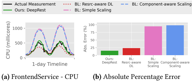
Figure 17. The estimation of the CPU utilization of the FrontendService in the hotel reservation system having 3× more users than ever.
