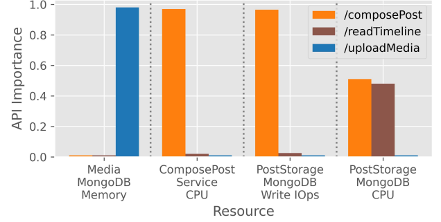
Figure 22. DeepRest neural design reveals the dependencies between resources and API endpoints.
