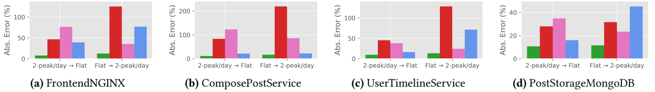
Figure 16. Estimating CPU utilization given query API traffic with unseen traffic shapes.
