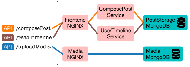
Figure 8. Three representative APIs and their simplified invocation relationships with six components in the social network application.
