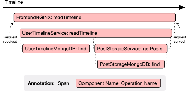
Figure 3. The execution diagram of a trace originated from a /readTimeline API request.
