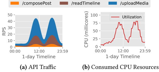
Figure 2. An example of one-day API traffic and its consumed CPU resources in the FrontendNGINX webserver.
