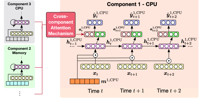
Figure 6. The API-aware DNN experts in DeepRest.
