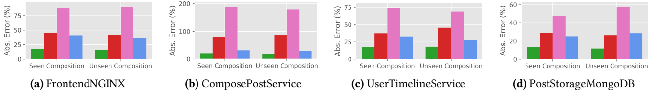
Figure 15. Estimating CPU utilization given query API traffic with unseen API compositions.
