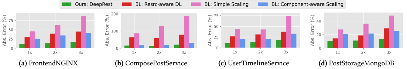
Figure 14. Estimating CPU utilization given query API traffic with unseen scales of application users.
