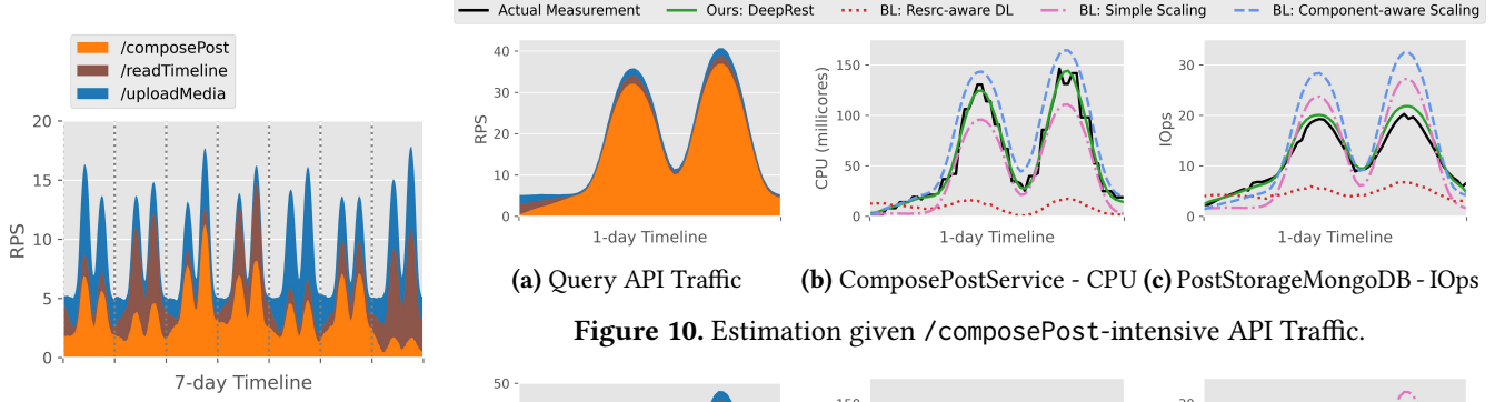
Figure 9. The 7-day API traffic during the application learning phase with three APIs: /composePost, /readTimeline, and /uploadMedia. Each day has two peak-hour (e.g., lunchtime and late evening) to match real-world social network behaviors.
