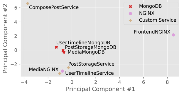
Figure 21. The DNN experts trained to estimate utilization in MongoDB components (red crosses) are similar to each other (forming a cluster).
