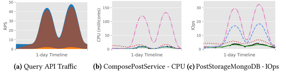
Figure 11. Estimation given /readTimeline-intensive API Traffic.
