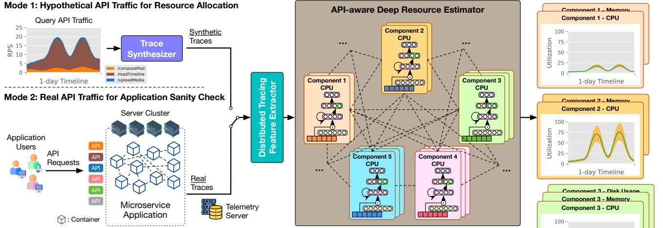
Figure 4. The end-to-end design of DeepRest with two modes in the query phase. The synthetic/real traces are sent to the feature extractor to transform them into structured features for the API-aware deep resource estimator to predict utilization.
