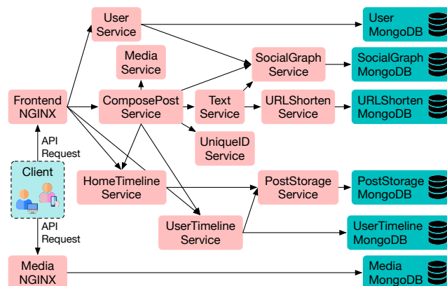
Figure 1. The flow of API requests across components in a social network application from DeathStarBench [30].
