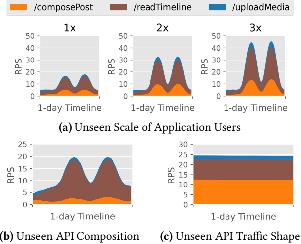
Figure 13. Examples of one-day query API traffic of the three types of queries in business scenarios.
