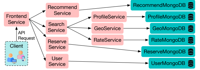
Figure 7. The hotel reservation application.
