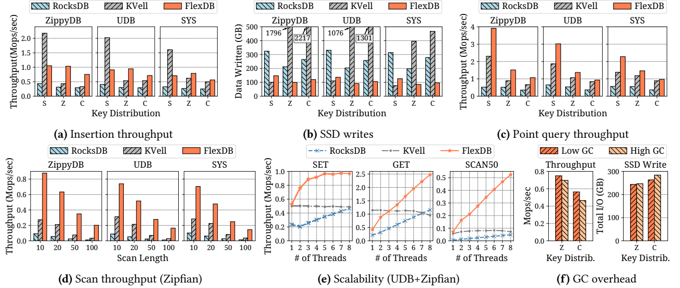
Figure 11. Microbenchmark results of FlexDB. Key distributions: S – Sequential; Z – Zipfian; C – Zipfian-Composite.
