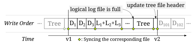
Figure 8. An example of write ordering in FlexSpace
