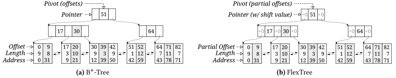
Figure 2. Examples of B + -Tree and FlexTree that manage the same address space
