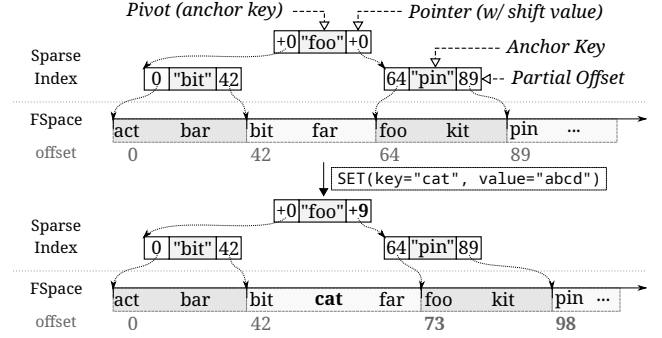
Figure 9. An example of the sparse KV index in FlexDB
