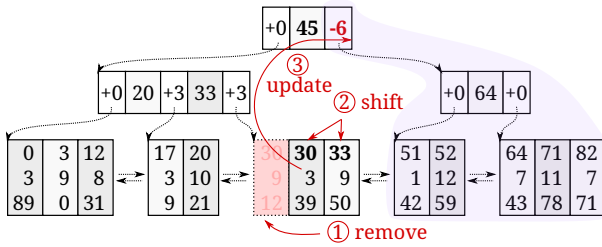
Figure 6. Removing address mapping from offset 33 to 42
