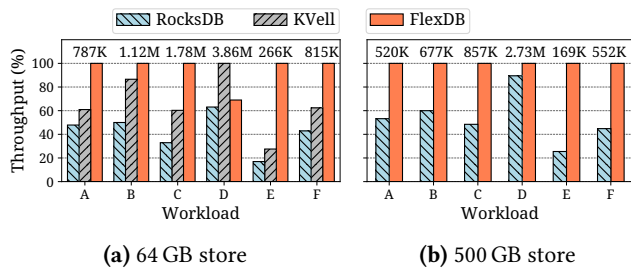
Figure 12. YCSB benchmark with the UDB KV data size. Results of each workload are normalized to the highest. The throughput (ops/sec) of the highest bar in each experiment is shown on the top.
