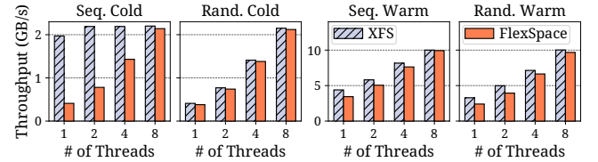
Figure 10. Read throughput after random write (4 KB)
