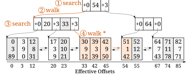
Figure 5. Looking up mappings from 36 to 55 in FlexTree
