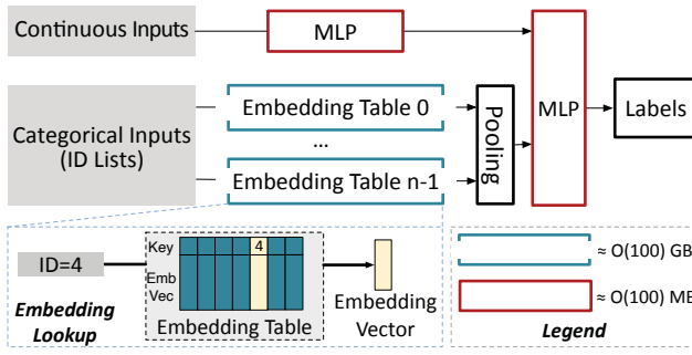
Figure 1. The structure of Deep Learning Recommendation Model (DLRM).
