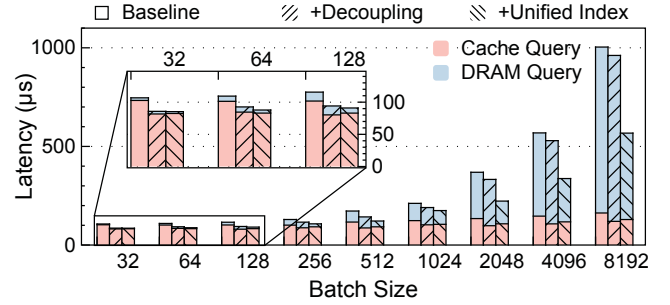
Figure 15. (Exp #7) Benefits of unified index and decoupling copying from indexing. Design techniques are cumulative. Baseline: HugeCTR with flat cache and self-identified kernel fusion. Decoupling: decoupling copying from indexing. Cache Query = Cache Index + Cache Copy, so is DRAM.
