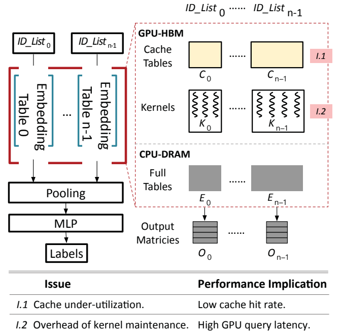
Figure 2. The sparse part of DLRM and the existing GPU-resident cache scheme.
