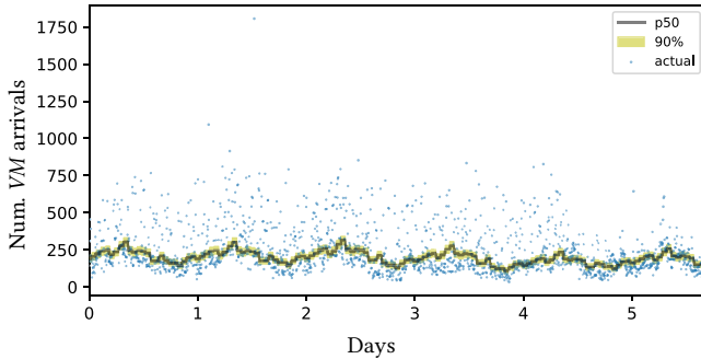
Figure 6. Actual and generated (with median, 90% prediction intervals) individual VM arrivals over Azure test window. Modeling raw job arrivals with Poisson greatly underestimates the variance in the arrival process (only 18% of true values are captured in the 90% prediction interval).
