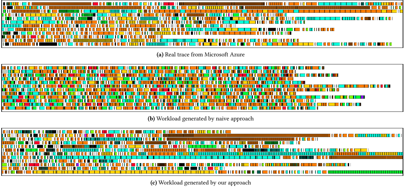
Figure 1. Workload/model visualization: Each rectangle represents a VM, each row shows all VM arrivals in one 5-minute period. Color represents VM flavor , width represents lifetime (compressed non-linearly to discrete bins; bin indices are used as width). Rows are not timelines showing when VMs start/stop, but rather depict resource and lifetime properties of VMs arriving sequentially in a period. In real workloads (and in those from our generator), VMs arrive in user-specific batches (space-separated here), within each batch VMs have similar properties, and arrival rates vary a lot from period to period.
