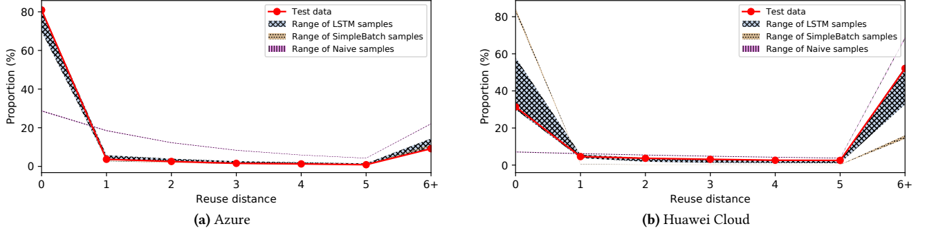
Figure 9. Reuse distance distributions for generated traces and actual data over Azure (9a) and Huawei Cloud (9b) test windows. LSTM traces are the only traces that consistently match the reuse pattern of actual test data across both clouds.
