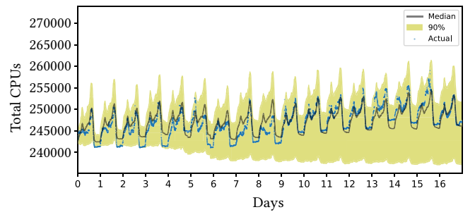
(c) LSTM-generated: 93% captured in 90% prediction interval
