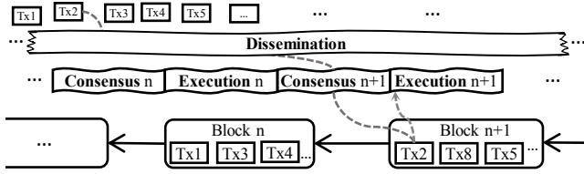
Figure 1. The DiCE (Dissemination-Consensus-Execution) distributed computing model.
