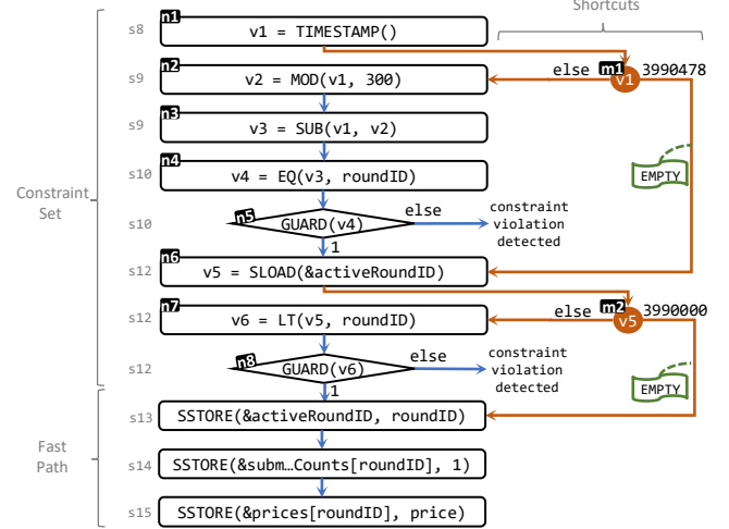
Figure 9. Accelerated program of Tx_e synthesized in FC4.
