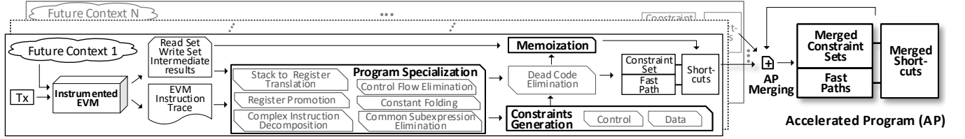
Figure 6. Workflow for synthesizing AP (Accelerated Program) via program specialization and memoization.
