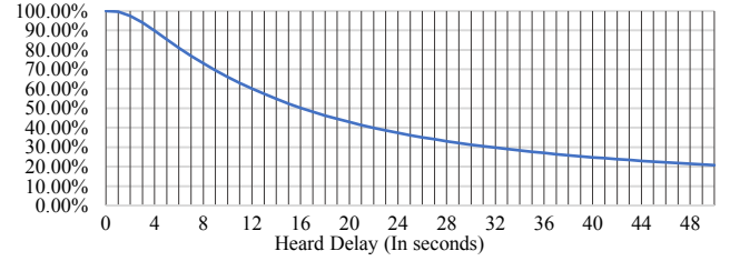
Figure 11. Reverse CDF of heard delay ( y percentage of heard transactions whose delay exceed x seconds).
