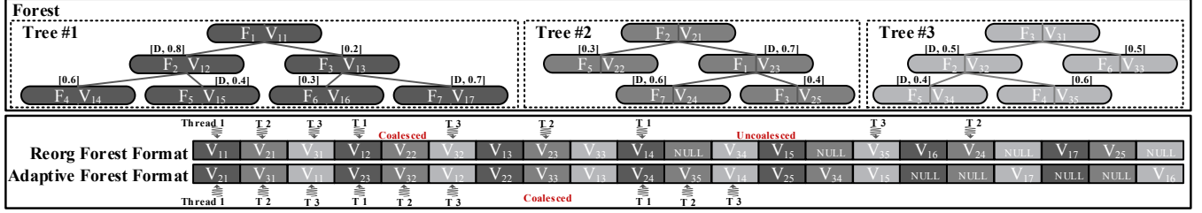
Figure 1. An example of decision tree ensemble and memory access sequences using the reorg forest format.
