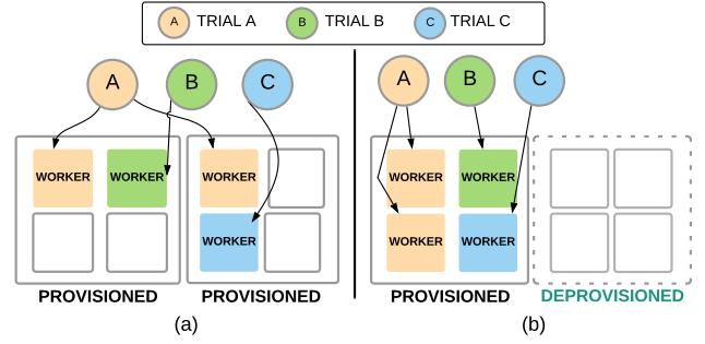
Figure 5. Worker location during hyperparameter tuning. A scattered placement of training workers across cluster resources can lead to low training throughput. By colocating workers and constraining the worker placement to use a minimal feasible set of nodes, nodes can be easily deprovisioned without interrupting the experiment, leading to more efficient spending.
