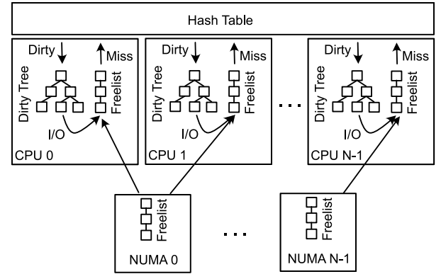
Figure 4. DRAM cache organization in Aquila .
