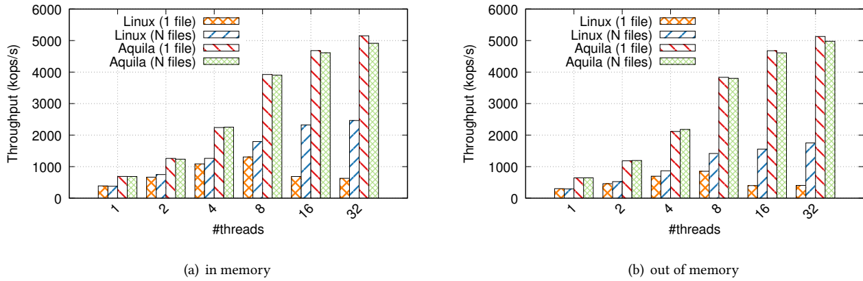
Figure 10. Scalability of Aquila vs. Linux mmap using random reads for both a shared and a private file per thread with (a) a dataset that fits in memory and (b) a dataset that does not fit in memory.
