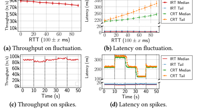
Figure 9. DAST’s performance on cross-region network anomalies.
