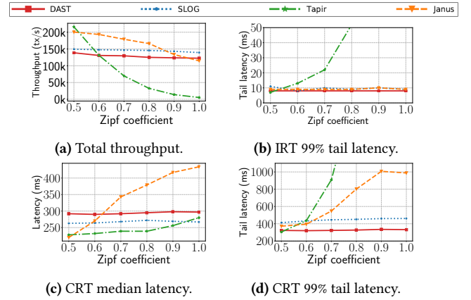
Figure 7. Performance on different conflict rates in the TPC-A workload (error bars omitted for readability).
