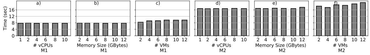
Figure 10. Scalability of InPlaceTP for KVM→Xen.
