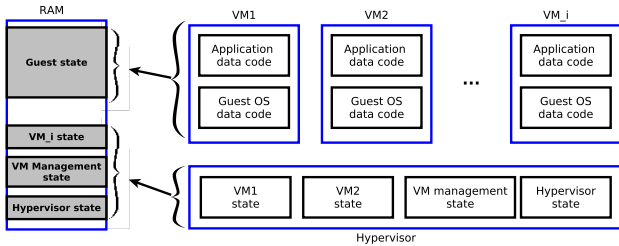
Figure 2. Memory separation organizes the content of the RAM in four categories: Guest State , VM i State , VM Management State and HV State .
