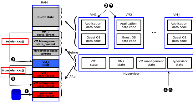
Figure 3. InPlaceTP workflow.
