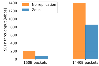
Figure 14. SCTP performance.
