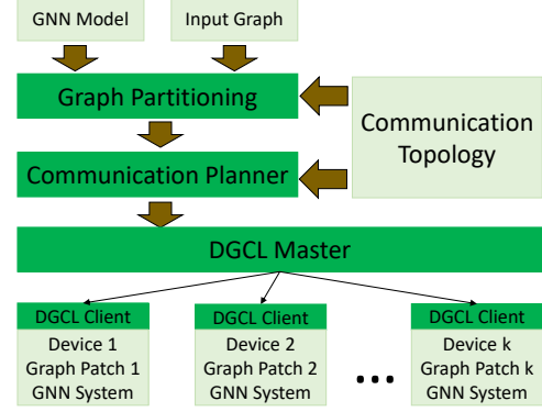
Figure 5. Architecture of DGCL
