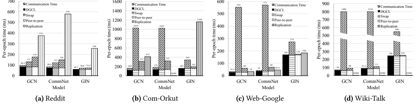
Figure 7. The per-epoch time and communication time for training the 3 GNN models on 4 datasets with 8 GPUs
