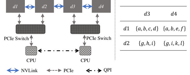
Figure 6. An example of communication topology and communication relation, in which d_1 and d_2 are senders
