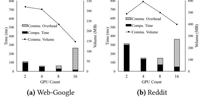
Figure 2. The computation time and communication overhead for training a 2-layer GCN with peer-to-peer communication (the average communication volume of each GPU during an epoch is plotted as dashed lines)
