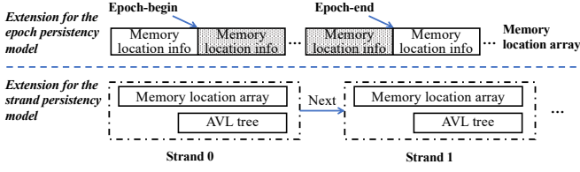
Figure 6: Extension to support a relaxed persistency model.
