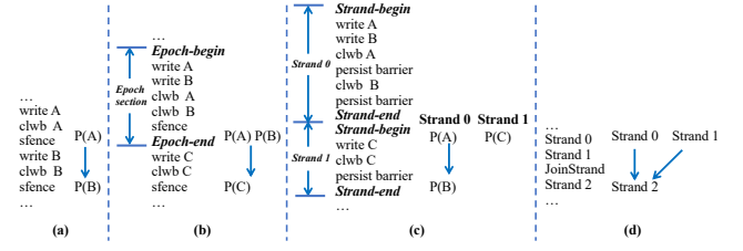
Figure 1: Examples of persistency models. P(x) means a write to x persists. The blue arrow specifies persist ordering: (a) strict persistency, (b) epoch persistency, (c) and (d) strand persistency.
