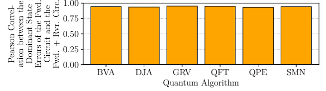
Figure 10: A high correlation exists between the dominant state error of the forward circuit and that of the forward + reverse circuit.
