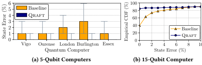
Figure 22: The median state error with QRAFT is 0% on (a) all 5-qubit computers and (b) the state error is also much lower than the Baseline on the 15-qubit Melbourne computer.
