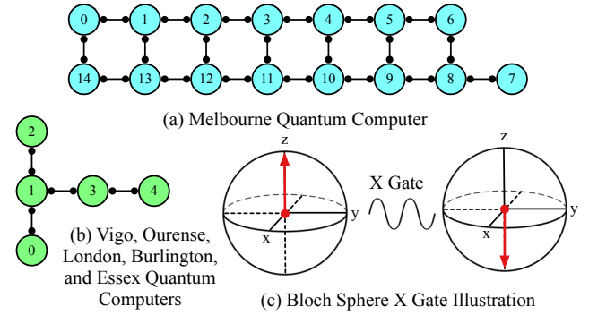
Figure 1: (a) Qubit connectivity layout of the 15-qubit Melbourne quantum computer. (b) Layout of the five-qubit quantum computers. (c) Bloch Sphere illustration of qubit state transformation using the X gate.
