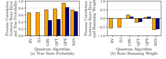
Figure 16: QRAFT reduces the error bias based on (a) true state probability, and (b) hamming weight for different algorithms.
