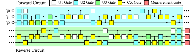
Figure 7: QFT's forward circuit (the upper half) is appended with the reversed version of it (the lower half) to construct the forward + reverse circuit.
