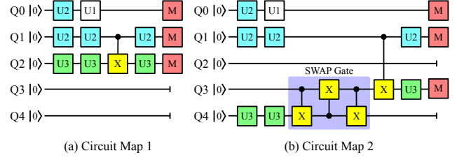
Figure 2: (a) Example of an optimal circuit map. (b) Sub-optimal circuit map that requires an extra SWAP operation.
