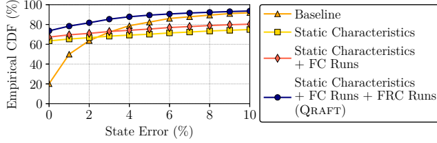
Figure 18: Training with the features generated using the forward + reverse runs (QRAFT) results in lower error than training using the features of just the forward runs or no runs at all.
