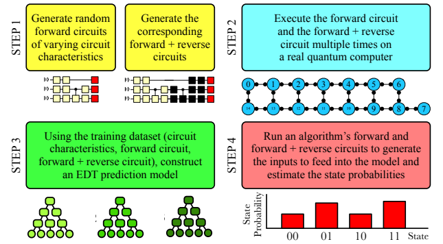
Figure 13: The steps taken for QRAFT's predictive model generation and inference.
