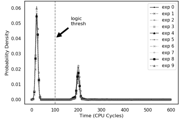
Figure 8: bp/icache OR Gate - Measured Timing KDE
