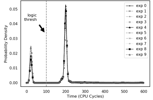
Figure 7: bp/icache AND Gate - Measured Timing KDE
