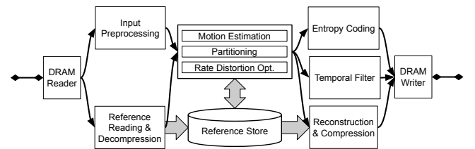
Figure 4: Encoder core functional pipeline
