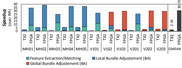
Figure 17: ORB SLAM speedup over RPi for TX2 and FPGA by category: feature extraction and bundle adjustments.
