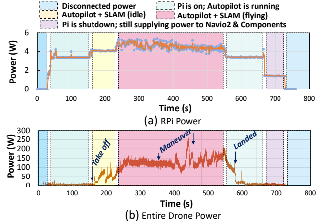
Figure 16: Power consumption graph of (a) RPi executing SLAM and autopilot code and (b) entire drone during flight.
