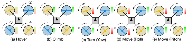
Figure 4: Essential drone movements. Colored rectangles near each rotor show how rotation speed changes, with red representing decrease and green representing increase.
