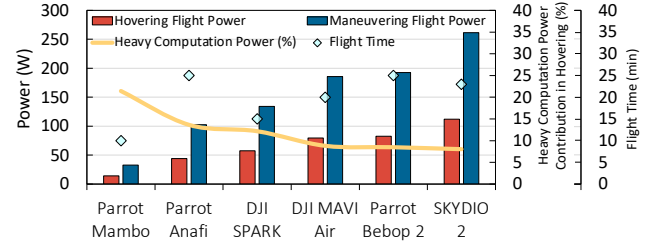
Figure 11: Commercial small-sized drones' heavy computation power contribution and their flight time.
