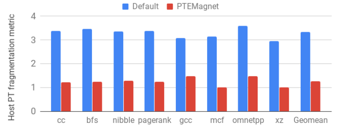
Figure 5: Host PT fragmentation in colocation with objdet (lower is better).
