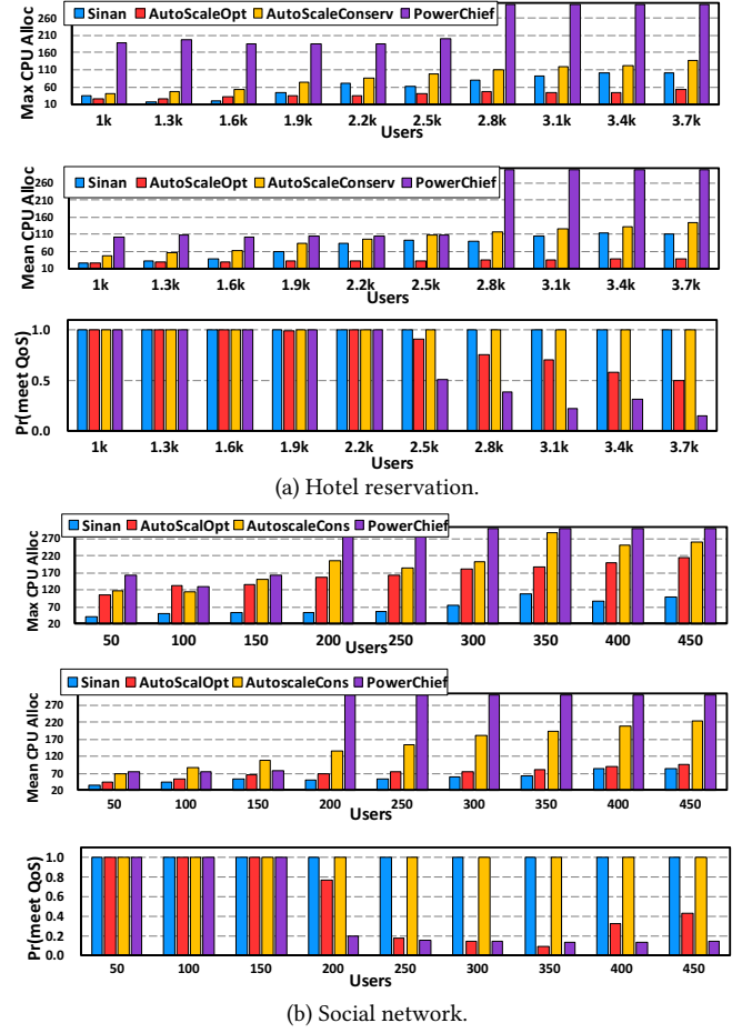
Figure 11: The mean and max CPU allocation, and the probability of meeting QoS for Sinan, Autoscaling, and PowerChief.
