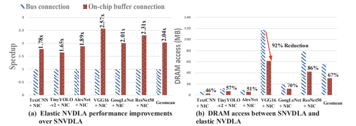
Figure 10. The performance improvement of tightly coupled DNN accelerator architecture
