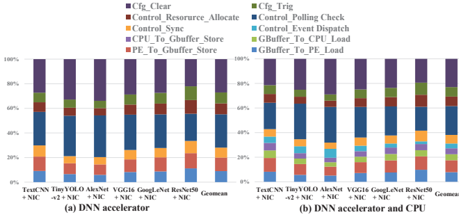
Figure 11. The Percentage of Different Instructions
