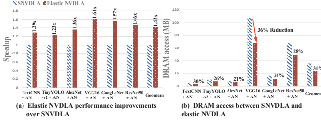
Figure 9. The Performance Comparison of Elastic NVDLA and SNVDLA
