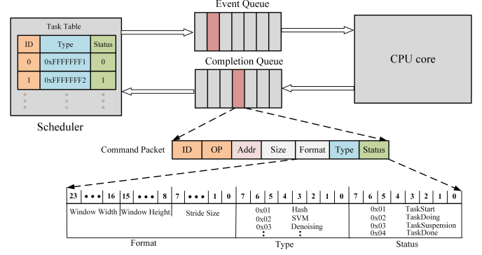
Figure 6. Event Queue Communication Mechanism
