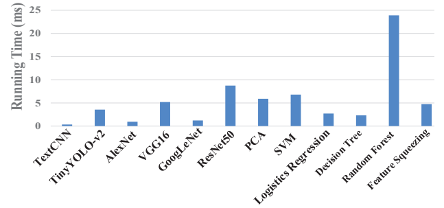
Figure 12. The Performance of Non-DNN Defence on CPU
