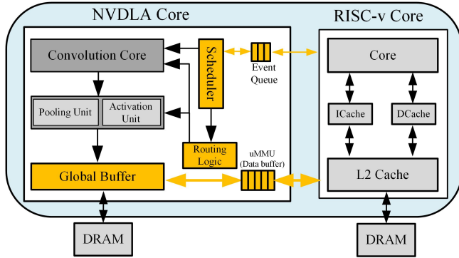
Figure 8. Elastic NVDLA and RISC-V implement DNNGuard architecture
