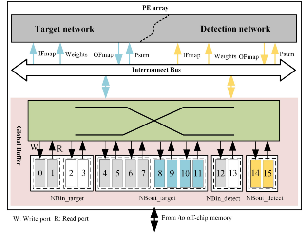
Figure 3. Elastic On-chip Buffer
