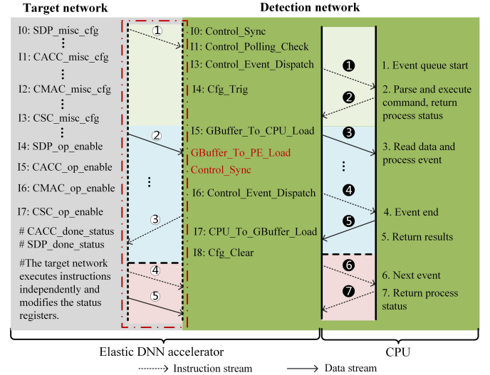
Figure 7. A Running Example of DNNGuard
