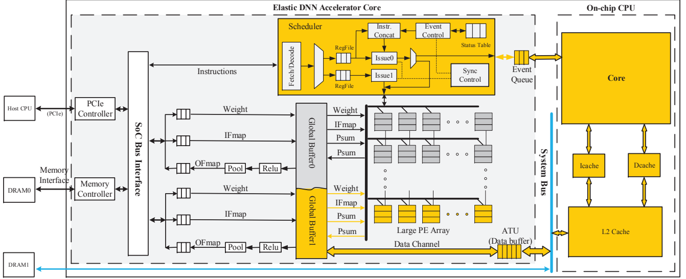
Figure 2. The DNNGuard Architecture Based on Elastic DNN Accelerator and CPU Core
