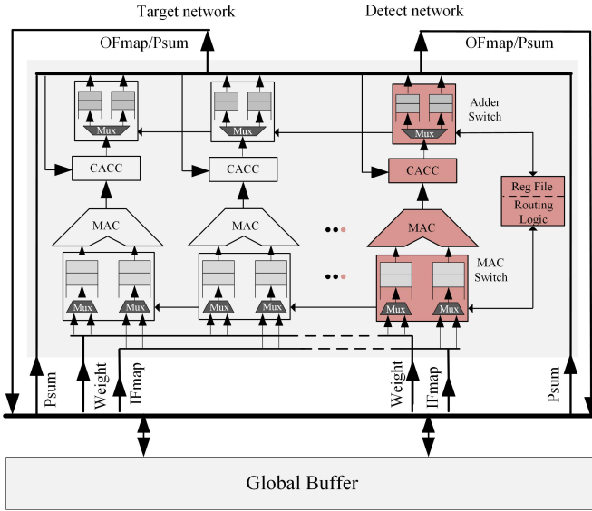
Figure 4. DNN Accelerator with Elastic PE Structure
