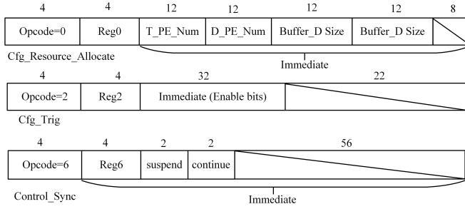
Figure 5. Extended AI Instruction Format
