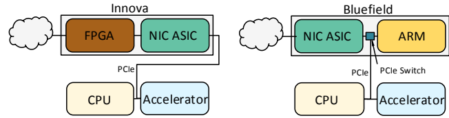
(a) Innova - FPGA bump in the wire (b) Bluefield - ARM multi host
