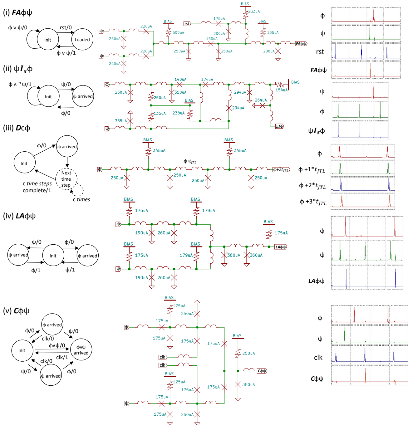
Figure 3. Panel (i): FIRSTARRIVAL \mathbf{FA}ab . Panel (ii): strict INHIBIT a\mathbf{I}_Sb . Panel (iii): DELAY \mathbf{D}ca , where t_{JTL} is the delay that each JTL causes. Panel (iv): LASTARRIVAL \mathbf{LA}ab . Panel (v): COINCIDENCE \mathbf{C}ab .
