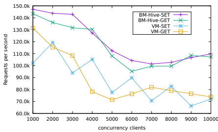
Figure 15. Redis with varying clients
