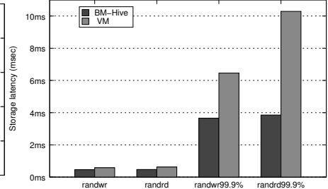
Figure 11. Storage I/O latency
