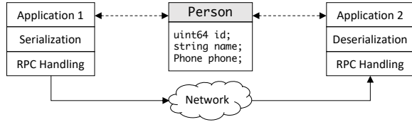
Figure 1. Two applications communicating using RPC.
