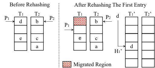
Figure 6. Example of the rehash operation.
