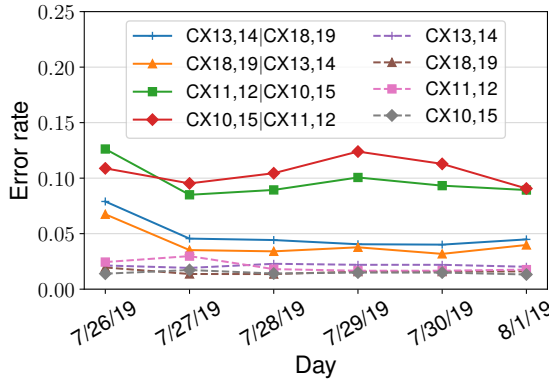
Figure 4. Daily variations of crosstalk noise in IBMQ Poughkeepsie. Lower error rate is better. Conditional error rates of a gate, say E(CX13,14|CX18,19) are much higher than the independent error rate throughout the experiment week. The conditional error rates vary up to 2x on this machine, and up to 3x across devices.
